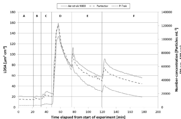
Fig. 7. Lung-deposited surface area concentration and number concentration of particles measured in a private house with operational wood-burning stove. A=baseline recording before start of experiment; B=ignition of stove; C=opening of stove due to extinguishing flame; D=boiling of water; E/F=fresh wood billets added to stove.
